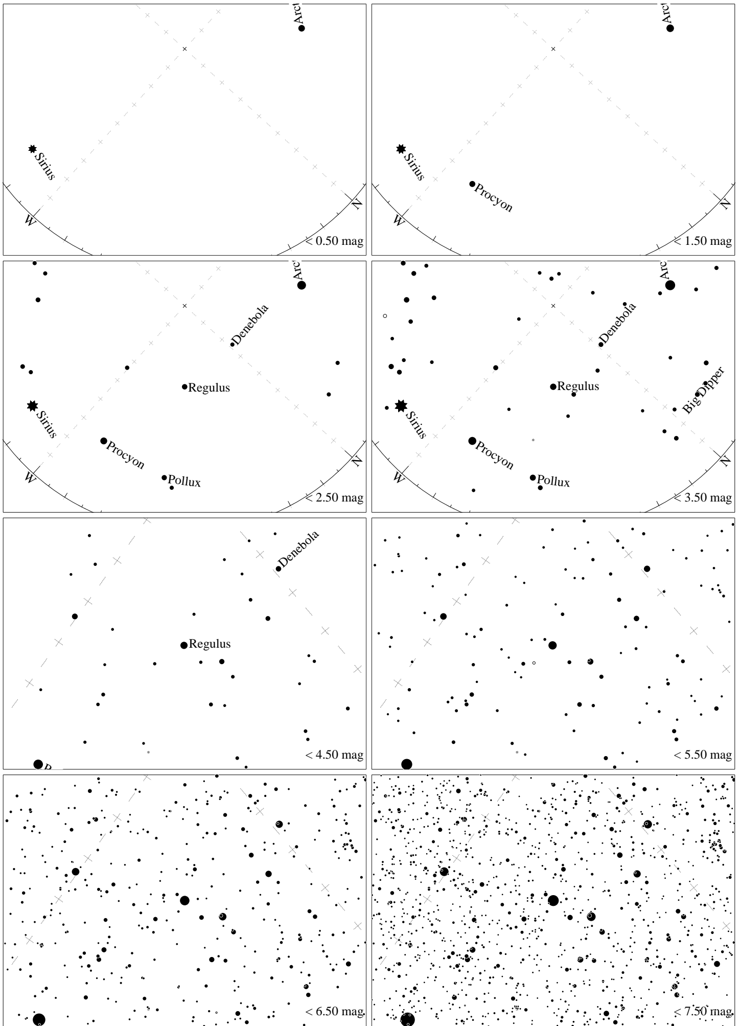
Maps for Globe at Night at latitude -10^\circ , 2024-05-02, 21 h local time (Sun at -47^\circ ), transparent air. Lines from N(E,S,W) to zenith shown (crosses each 10^\circ ). Regulus ( \alpha Leonis) is 48^\circ to the left from N, at 58^\circ height. Detailed maps 50^\circ vertically, the first four maps 100^\circ . Jan Hollan maps, CzechGlobe
