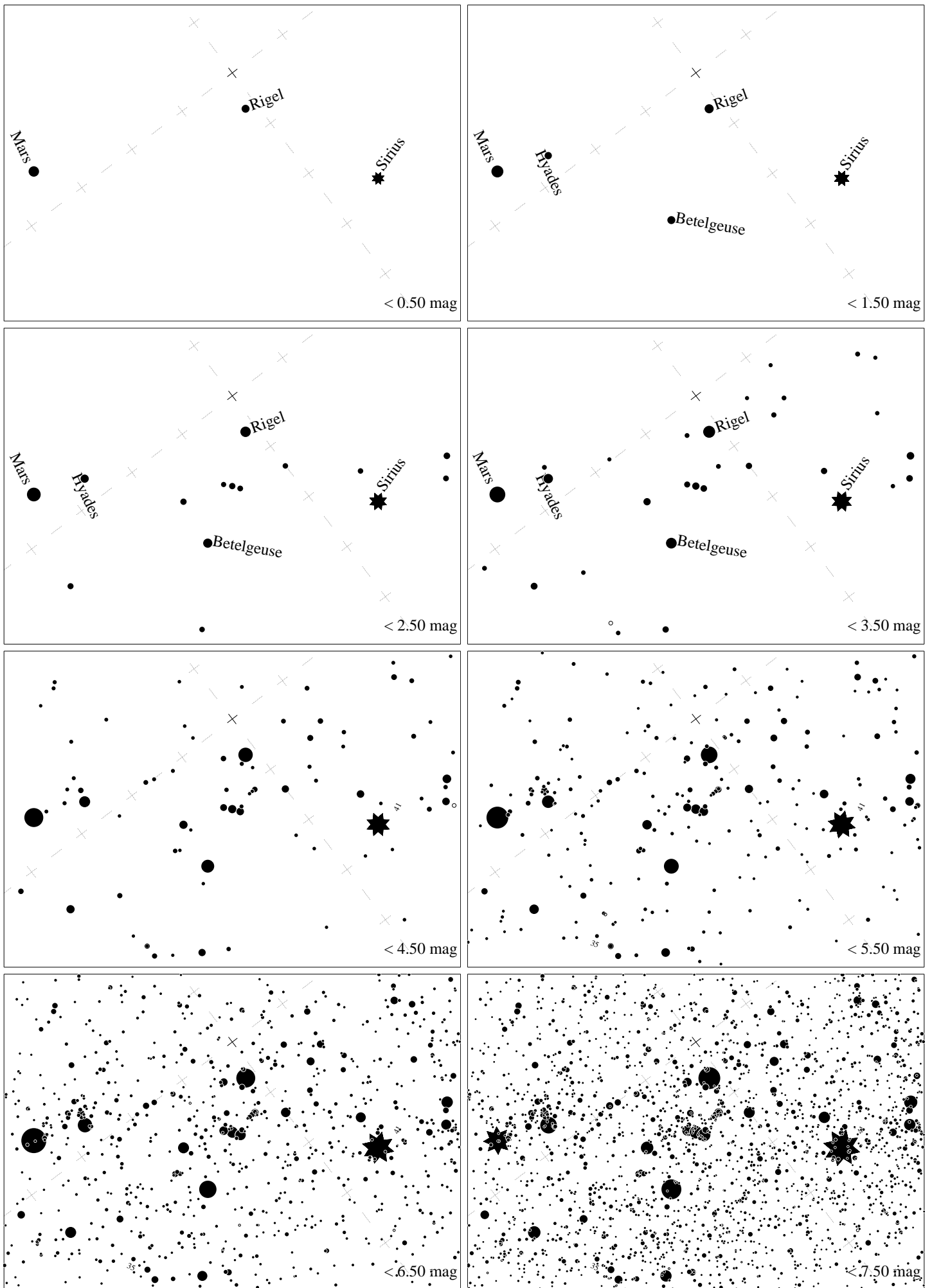
Maps for Globe at Night at latitude -10^\circ , 2023-01-18, 21 h local time (Sun at -34^\circ ), transparent air. Lines from N(E,S,W) to zenith shown (crosses each 10^\circ ). Orion's belt is 53^\circ to the right from N, at 76^\circ height. Star clusters M 41 and M35 marked when appropriate. Map vertical size is 50^\circ . Jan Hollan maps, CzechGlobe
