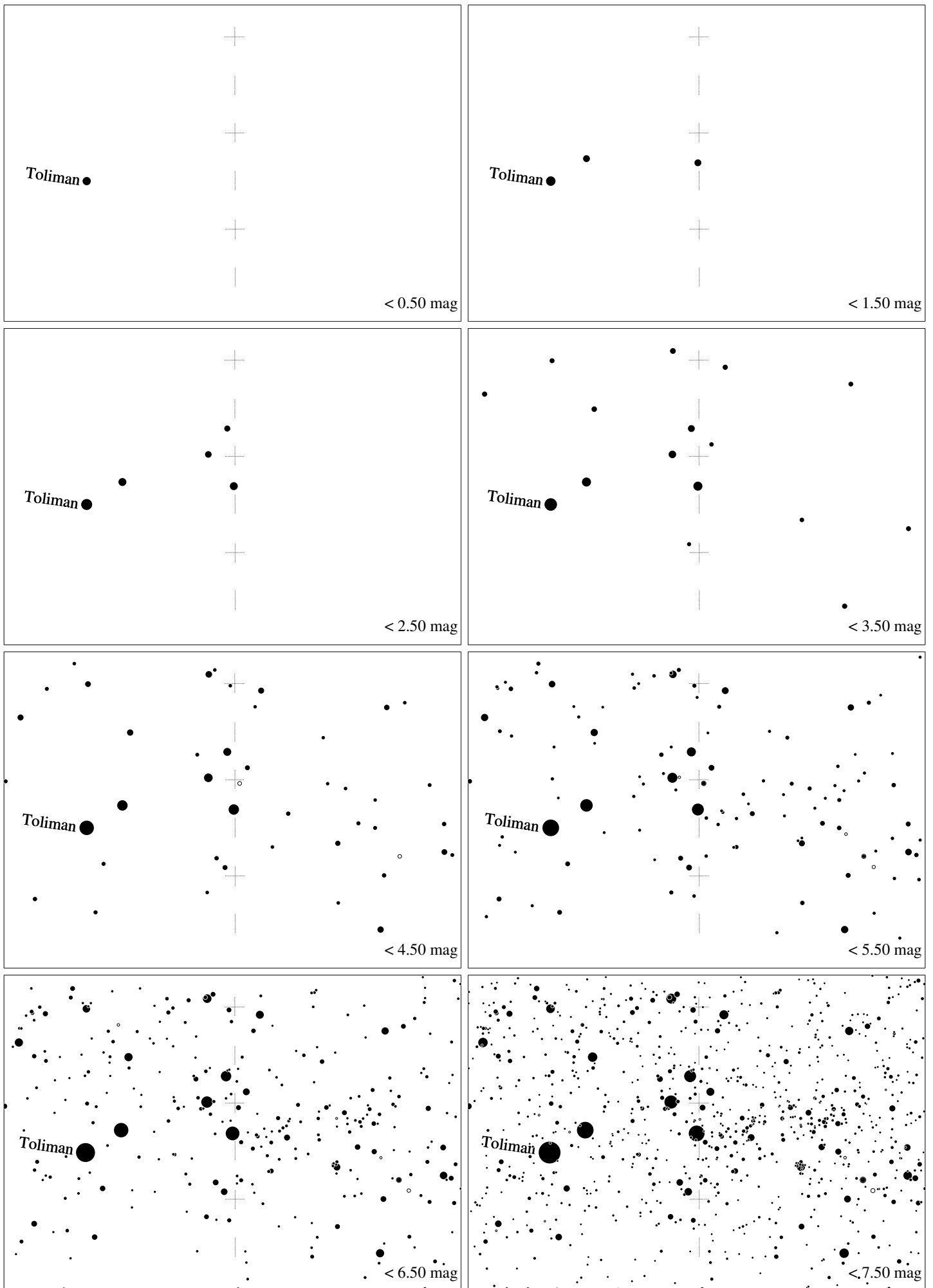
Maps for Globe at Night latitude 0°, 2015-05-13, 21 h local time (Sun at -43^\circ ), transparent air. The brightest star is Toliman ( \alpha Centauri). Central star Acrux (the brightest one in the Cross) is 0^\circ left from the south, at 27^\circ height. Map vertical size 33^\circ . Jan Hollan, CzechGlobe
