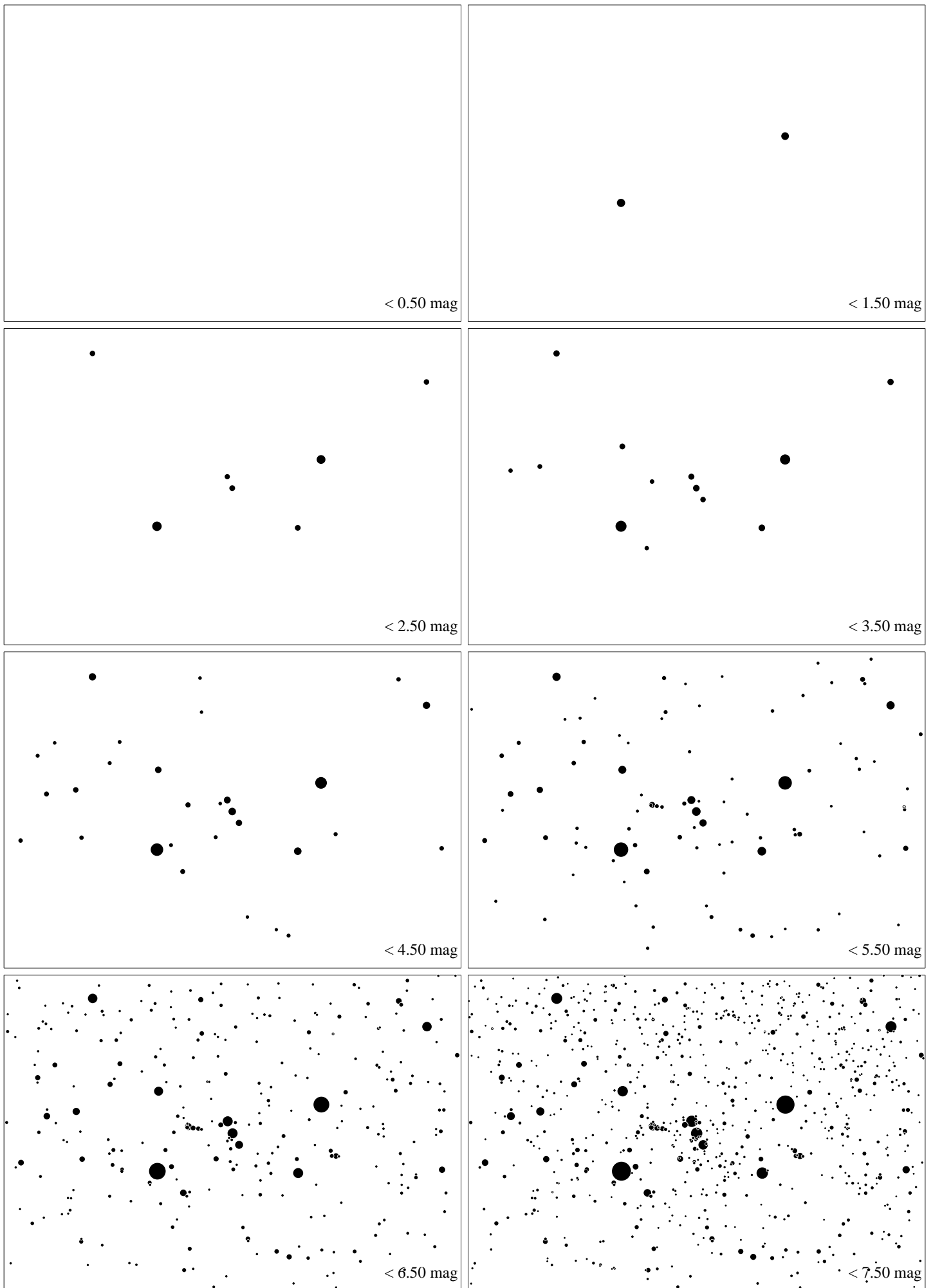
Maps for GLOBE at Night at latitude -10^\circ , March 30, 21 h local time (Mar 7, 22.5 h; Mar 23, 21.5 h, Apr 6, 20.5 h). Orion's belt is 95^\circ to the right from the south, at 31^\circ height. The brightest fixed star, Sirius, is just above the map at left. Jan Hollan, Ecological Institute Veronica and http://www.astro.cz/darksky
