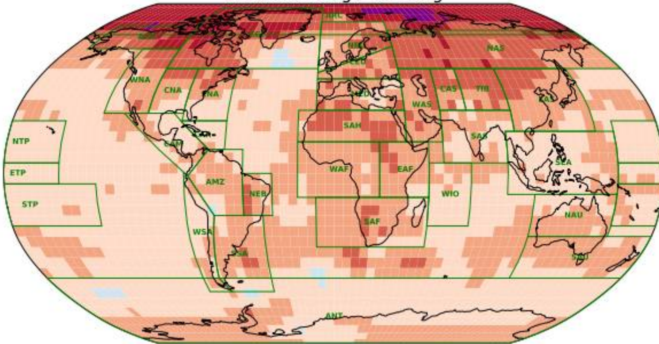
Annual average warming
