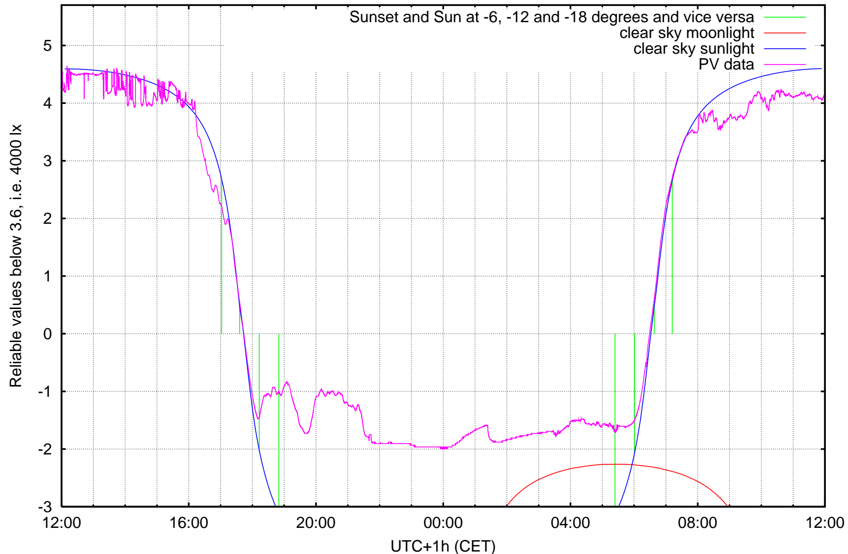
log10 ( illuminance / 1 lx ) Kravi hora, Brno, ending at Saturday 2007-02-10 noon
