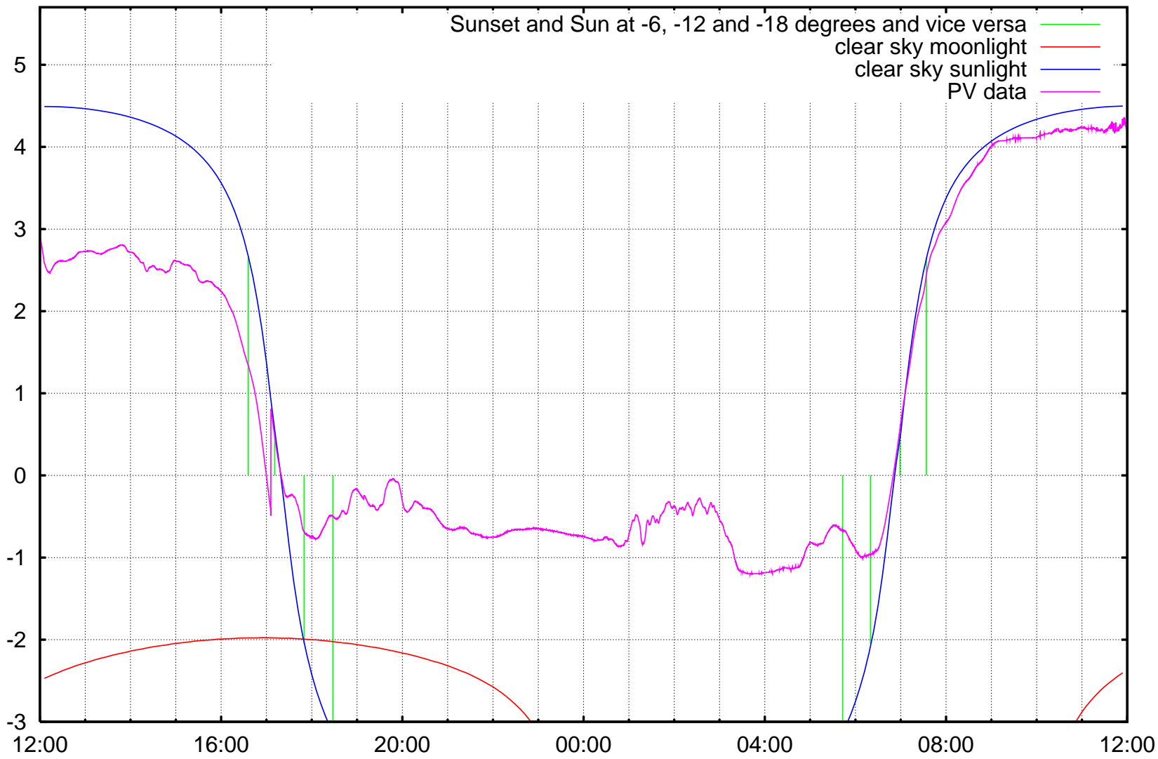
log10 ( illuminance / 1 lx ) Kravi hora, Brno, ending at Thursday 2007-01-25 noon
