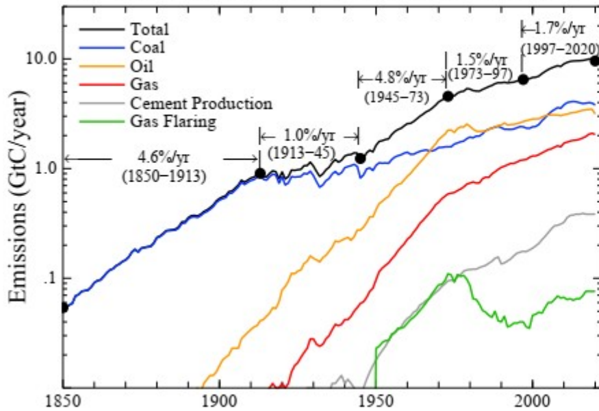
(a) Global Fossil-Fuel CO 2 Annual Emissions
