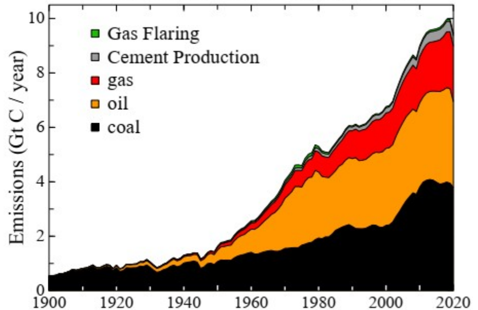
(b) Global Fossil-Fuel CO 2 Emissions
