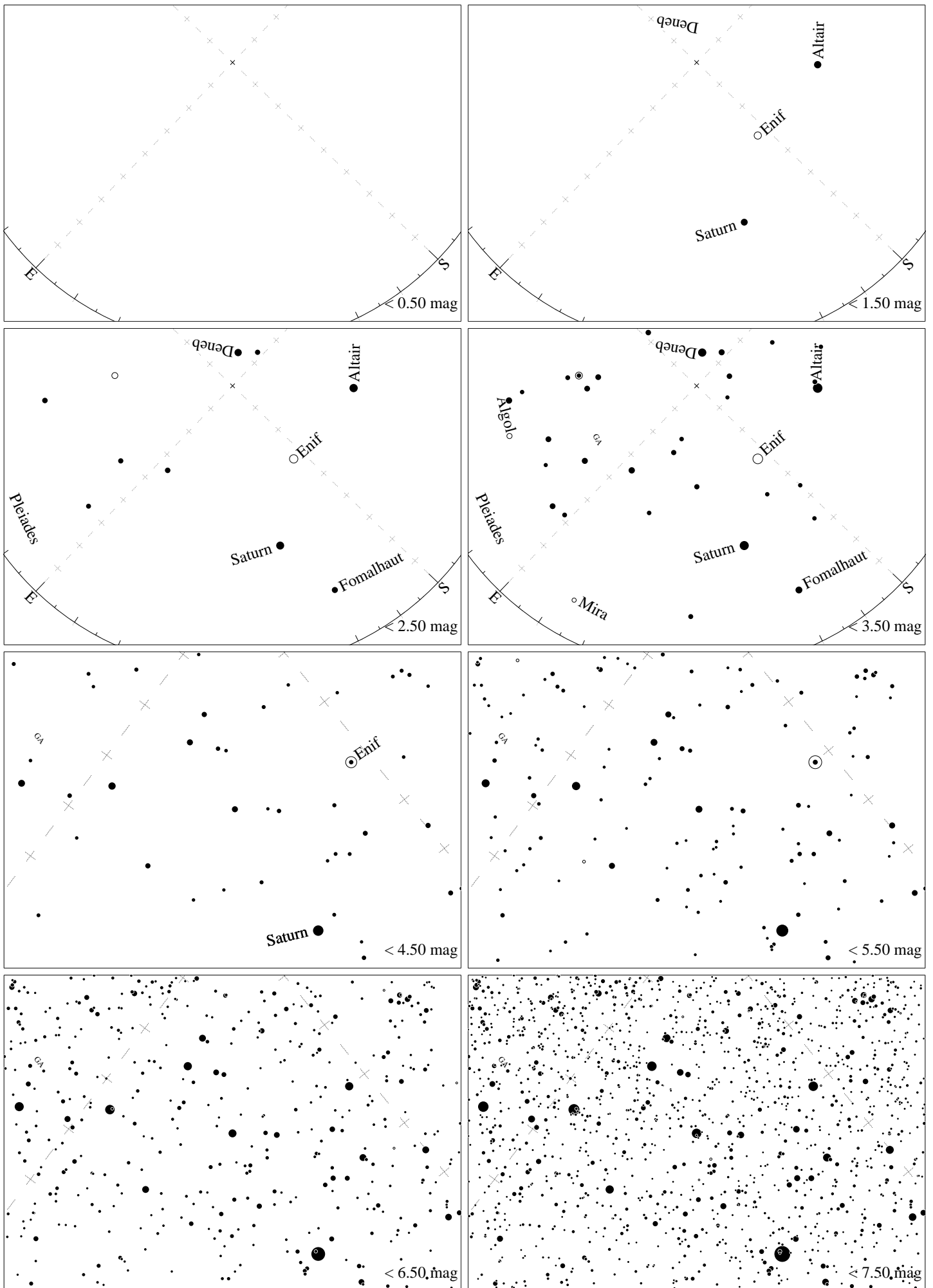
Maps for Globe at Night latitude 40°, 2024-09-28, 21 h local time (Sun at -36^\circ ), transparent air. Lines from N(E,S,W) to zenith shown (crosses each 10^\circ ). The map is centered on Markab ( \alpha Pegasi), which is 46^\circ to the left from S, at 58^\circ height. Detailed maps 50^\circ vertically, the first four maps 100^\circ . Jan Hollan, CzechGlobe
