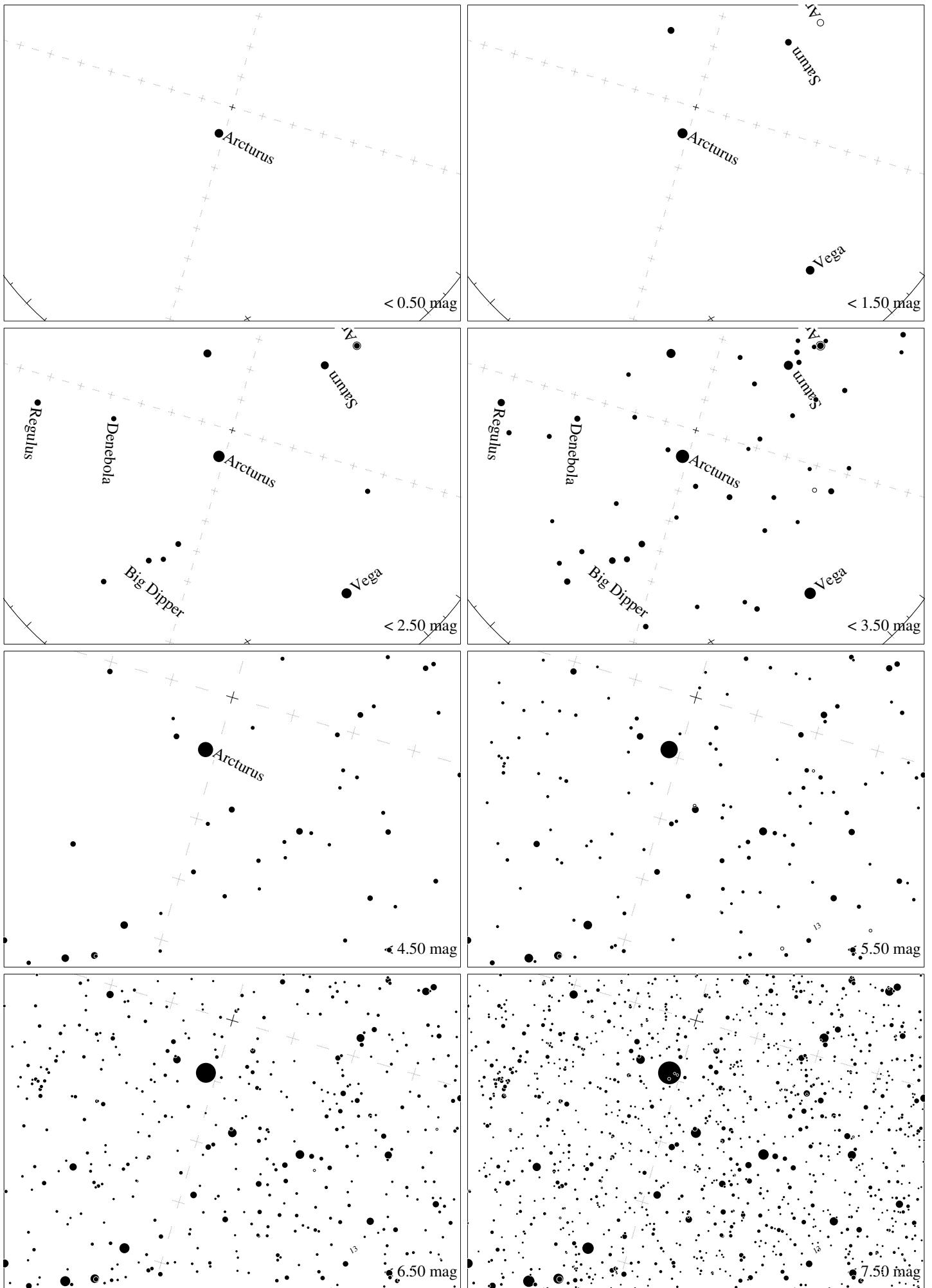
Maps for Globe at Night latitude 10^\circ , 2015-06-12, 21 h local time (Sun at -35^\circ ), transparent air. Lines from N(E,S,W) to zenith shown (crosses each 10^\circ ). Centered on Izar ( \epsilon Bootis), which is 16^\circ to the right from N, at 72^\circ height. Detailed maps 50^\circ vertically, the first four maps 100^\circ . Jan Hollan, CzechGlobe
