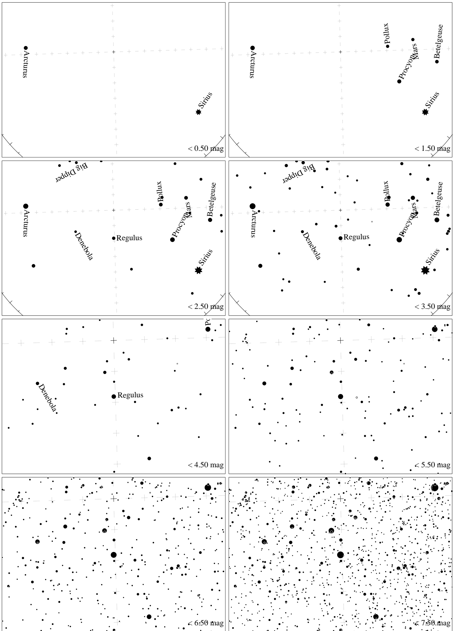
Maps for Globe at Night at latitude 30°, 2023-04-08, 21 h local time (Sun at -33°), transparent air. Lines from N(E,S,W) to zenith shown (crosses each 10°). Regulus ( \alpha Leonis) is 2° to the left from S, at 72° height. Detailed maps 50° vertically, the first four maps 100°. Jan Hollan maps, CzechGlobe
