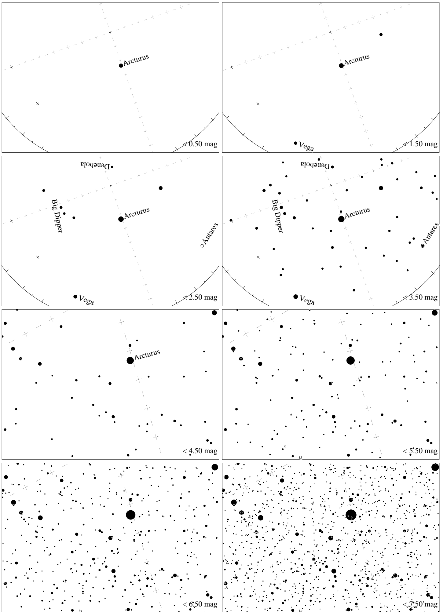
Maps for Globe at Night latitude 20^\circ , 2023-05-16, 21 h local time (Sun at -32^\circ ), transparent air. Lines from N(E,S,W) to zenith shown (crosses each 10^\circ ). Centered on Izar ( \epsilon Bootis), which is 70^\circ to the right from N, at 60^\circ height. Detailed maps 50^\circ vertically, the first four maps 100^\circ . Jan Hollan, CzechGlobe
