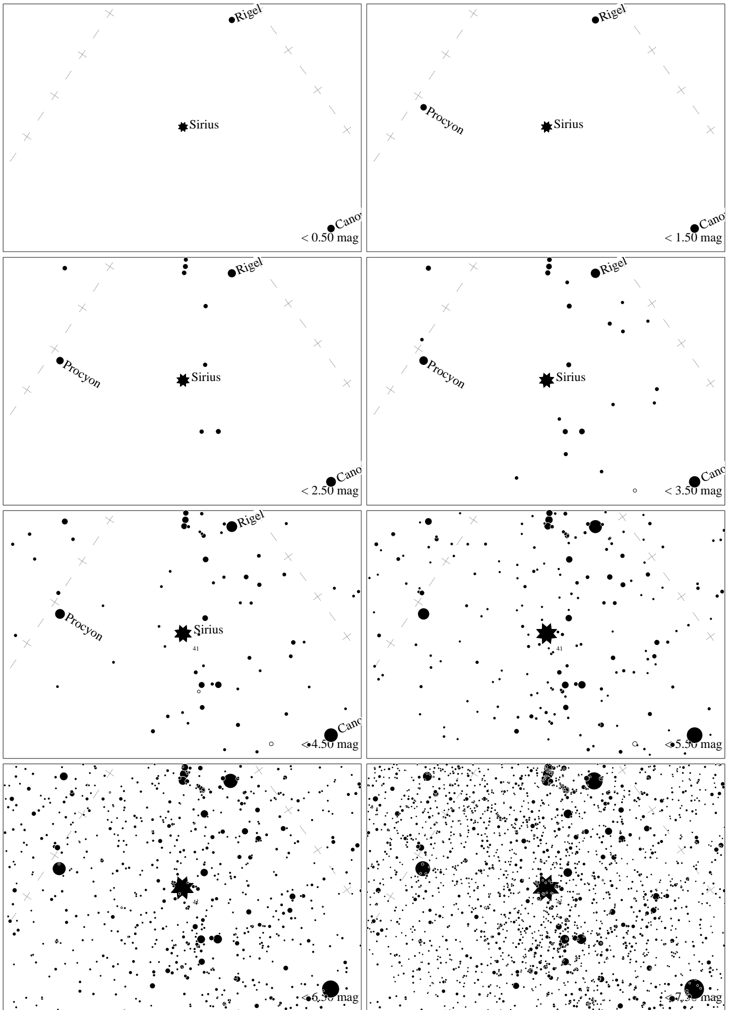
Maps for Globe at Night at latitude 10°, 2022-01-18, 21:00 local time (Sun at -43^\circ ), transparent air. Lines from N(E,S,W) to zenith shown (crosses each 10°). The brightest fixed star Sirius is 47^\circ to the left from S, at 51^\circ height. Star cluster M 41 marked when appropriate. Map vertical size is 50^\circ . Jan Hollan, CzechGlobe
