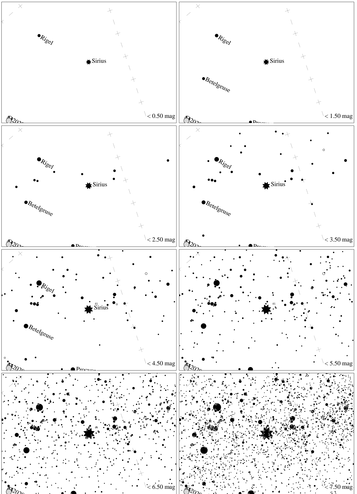
Maps for Globe at Night at latitude -40^\circ , 2020-01-09, 21 h local time (Sun at -14^\circ ), transparent air. Lines from N(E,S,W) to zenith shown (crosses each 10^\circ ). The brightest fixed star Sirius is 65^\circ to the right from N, at 50^\circ height. Star cluster M 41 marked when appropriate. Map vertical size is 50^\circ . Jan Hollan, CzechGlobe
