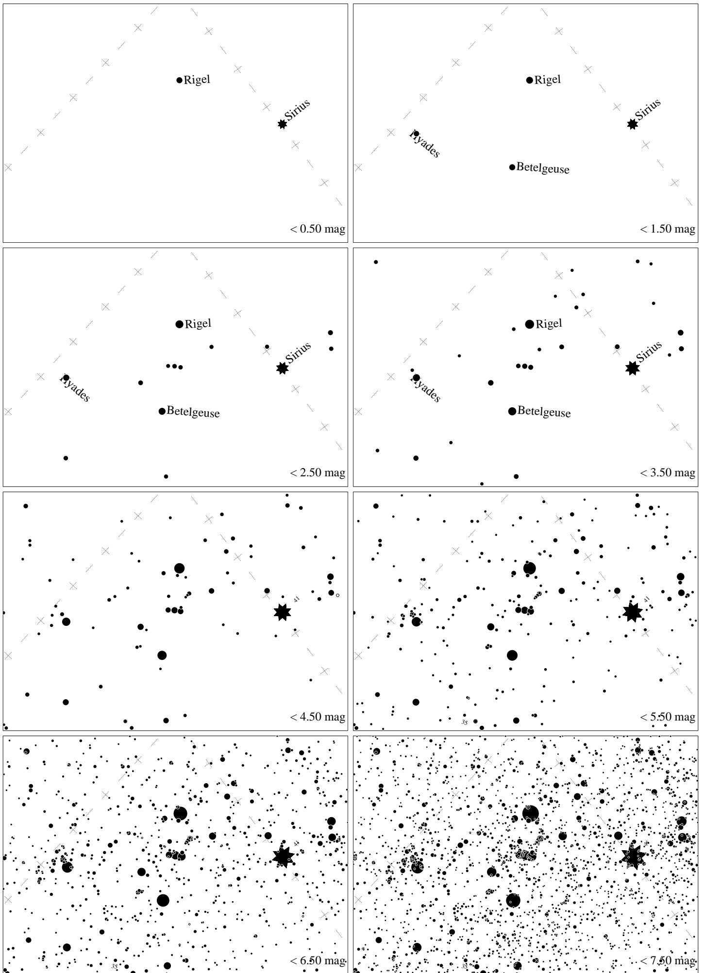
Maps for Globe at Night at latitude -20^\circ , 2021-01-09, 21 h local time (Sun at -28^\circ ), transparent air. Lines from N(E,S,W) to zenith shown (crosses each 10^\circ ). Orion 's belt is 48^\circ to the right from N, at 63^\circ height. Star clusters M 41 and M35 marked when appropriate. Map vertical size is 50^\circ . Jan Hollan maps, CzechGlobe
