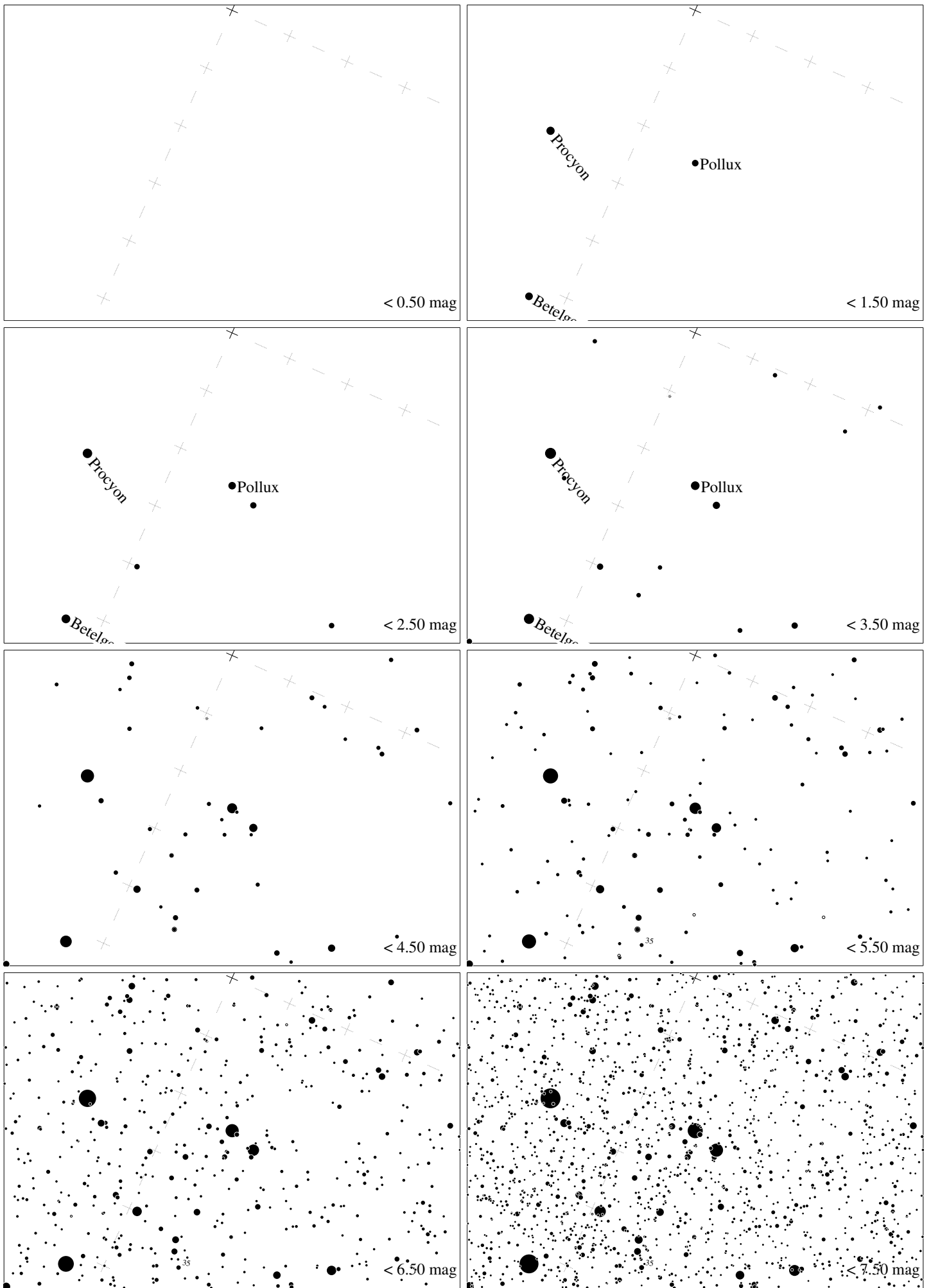
Maps for Earth Hour 2020 at latitude 20^\circ , 2020-03-28, 21 h local time (Sun at -39^\circ ), transparent air. Lines from N(E,S,W) to zenith shown (crosses each 10^\circ ). Pollux is 66^\circ to the left from N, at 66^\circ height. Star cluster M35 marked when appropriate. Map vertical size is 50^\circ . Jan Hollan maps, CzechGlobe
