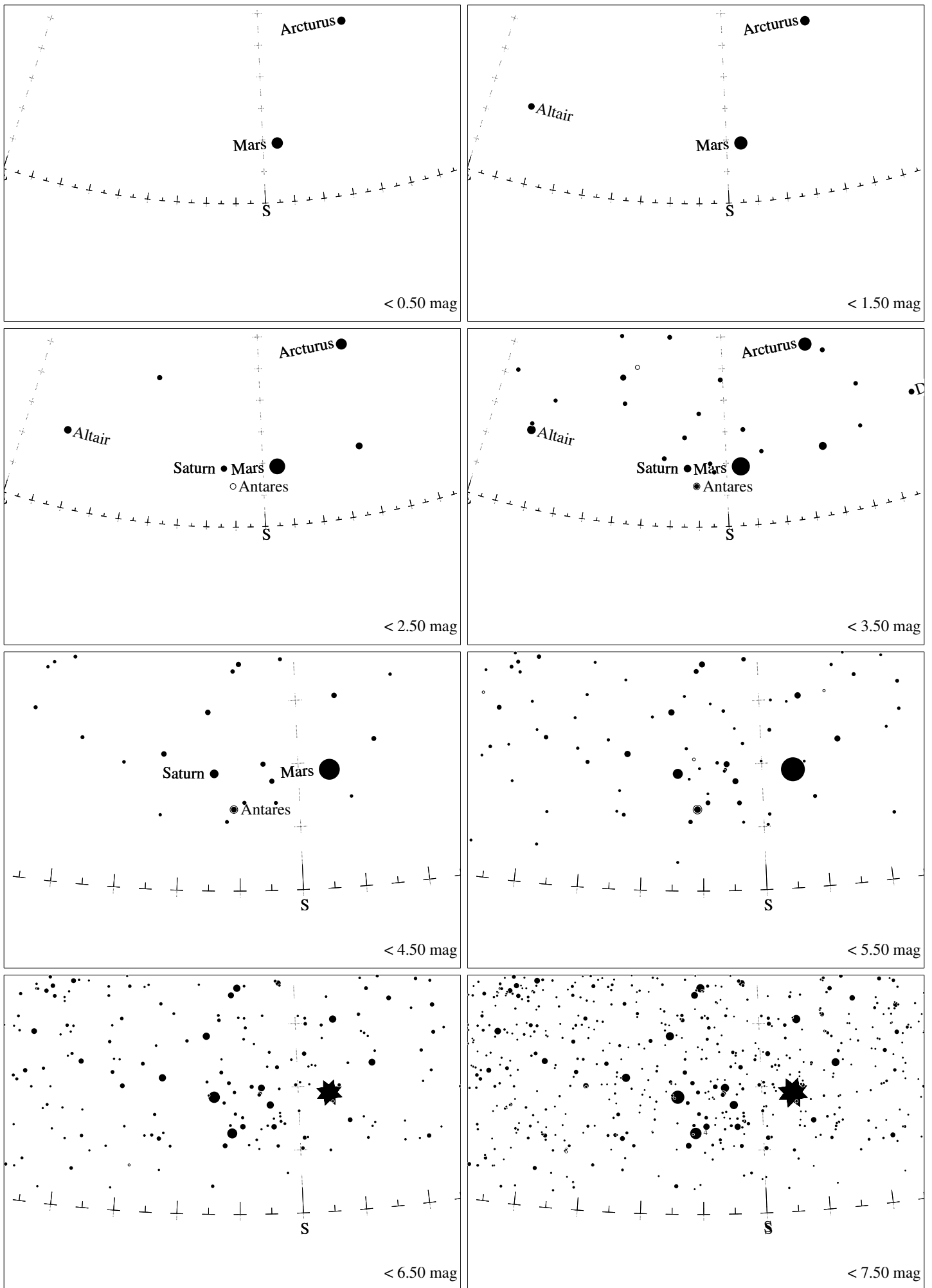
Maps for Globe at Night latitude 50°, 2016-07-01, 21 h local time (Sun at -6^\circ ), transparent air. Lines from N(E,S,W) to zenith shown (crosses each 10°). Centered on Antares ( \alpha Scorpii), which is 11^\circ to the left from S, at 13^\circ height. Detailed maps 50^\circ vertically, the first four maps 100^\circ . Jan Hollan, CzechGlobe
