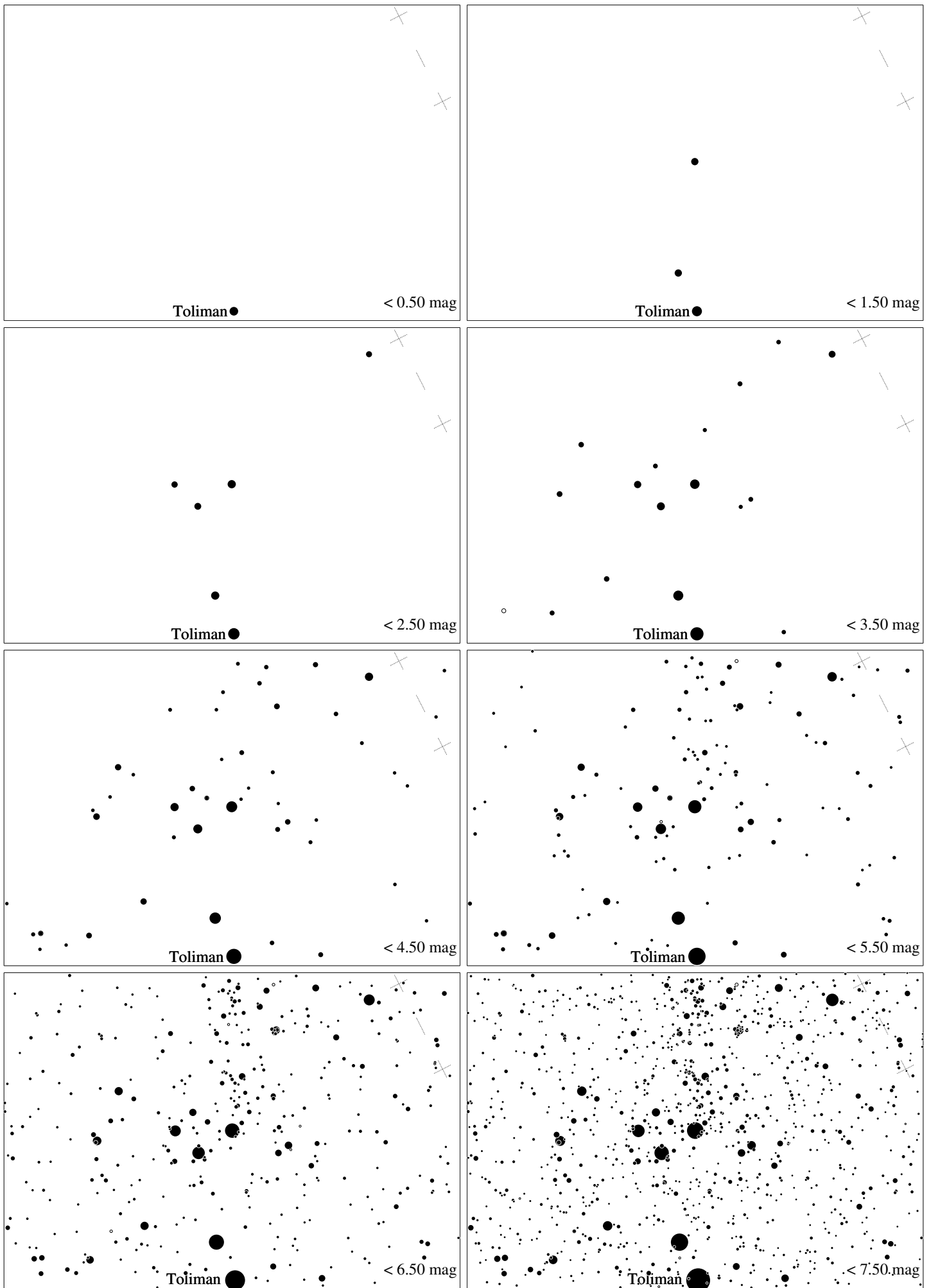
Maps for Globe at Night latitude -40^\circ , 2015-03-15, 21 h local time (Sun at -30^\circ ), transparent air. The brightest star is Toliman ( \alpha Centauri). Central star Acrux (the brightest one in the Cross) is 36^\circ left from the south, at 49^\circ height. Map vertical size 33^\circ . Jan Hollan, CzechGlobe
