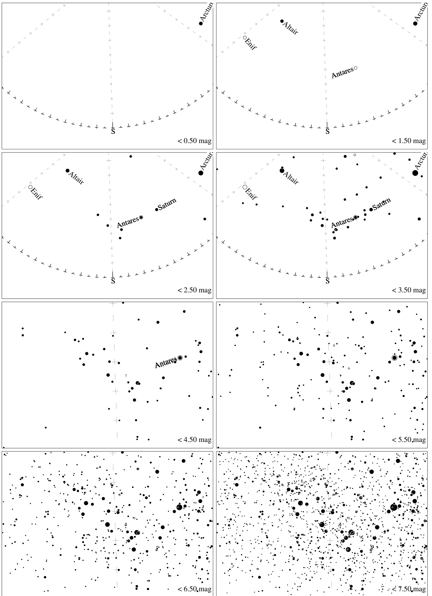
Maps for Globe at Night latitude 20°, 2015-08-09, 21 h local time (Sun at -32^\circ ), transparent air. Lines from N(E,S,W) to zenith shown (crosses each 10°). Centered on Kaus Australis ( \epsilon Sagittarii), which is 3° to the left from S, at 36° height. Detailed maps 50° vertically, the first four maps 100°. Jan Hollan, CzechGlobe
