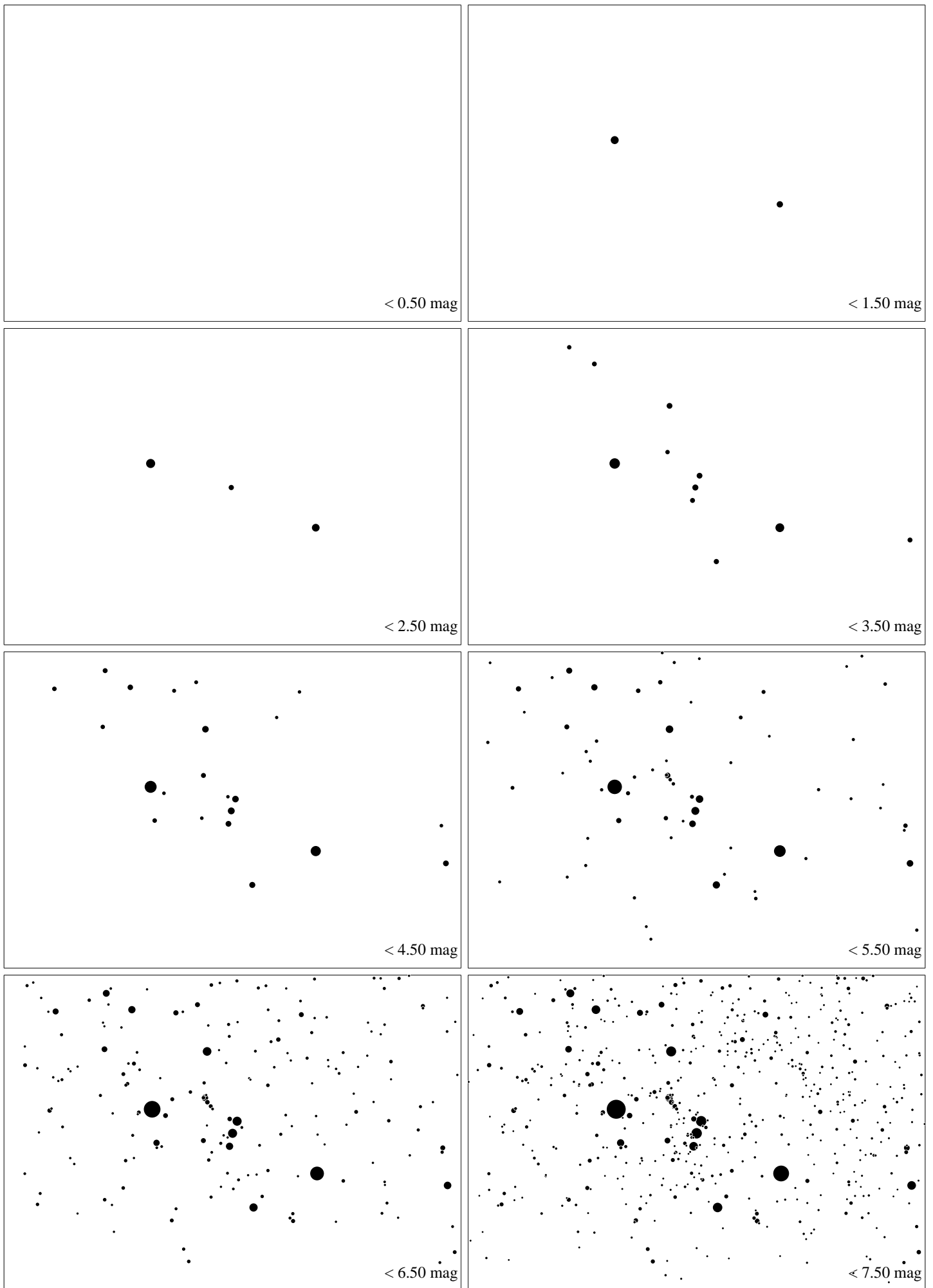
Maps for GLOBE at Night at latitude -50^\circ , March 30, 21 h local time (Mar 7, 22.5 h; Mar 23, 21.5 h, Apr 6, 20.5 h). Orion's belt is 114^\circ to the right from the south, at 21^\circ height. The brightest fixed star, Sirius, is a bit above the map. Jan Hollan, Ecological Institute Veronica and http://www.astro.cz/darksky
