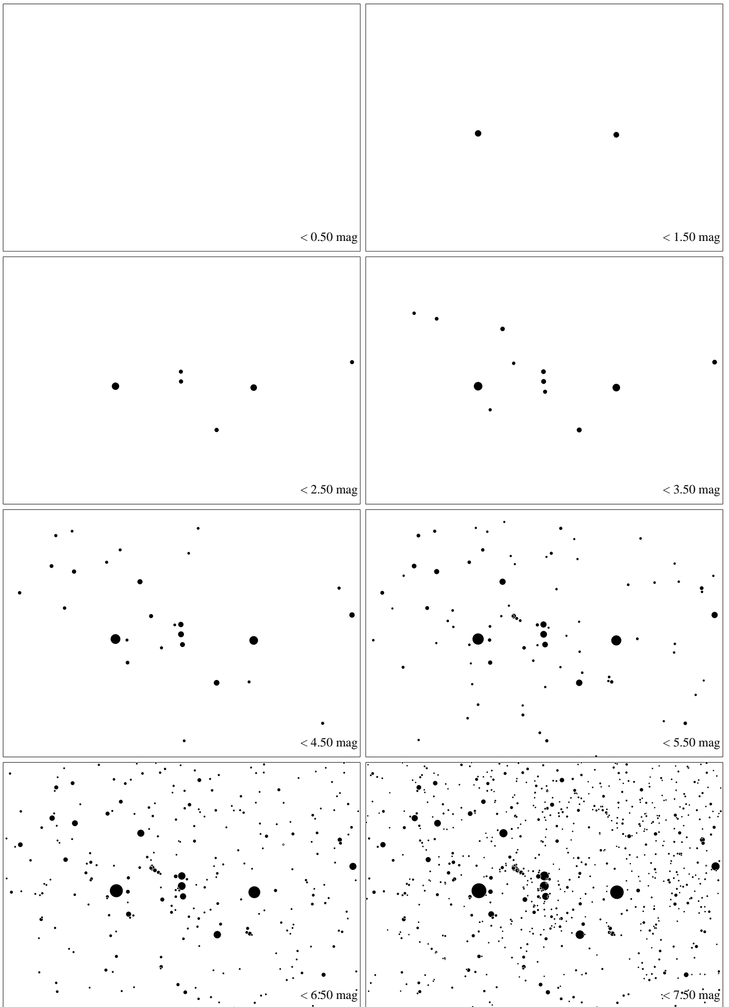
Maps for GLOBE at Night at latitude -30^\circ , March 30, 21 h local time (Mar 7, 22.5 h; Mar 23, 21.5 h, Apr 6, 20.5 h). Orion's belt is 106^\circ to the right from the south, at 27^\circ height. The brightest fixed star, Sirius, is a bit above the map. Jan Hollan, Ecological Institute Veronica and http://www.astro.cz/darksky
