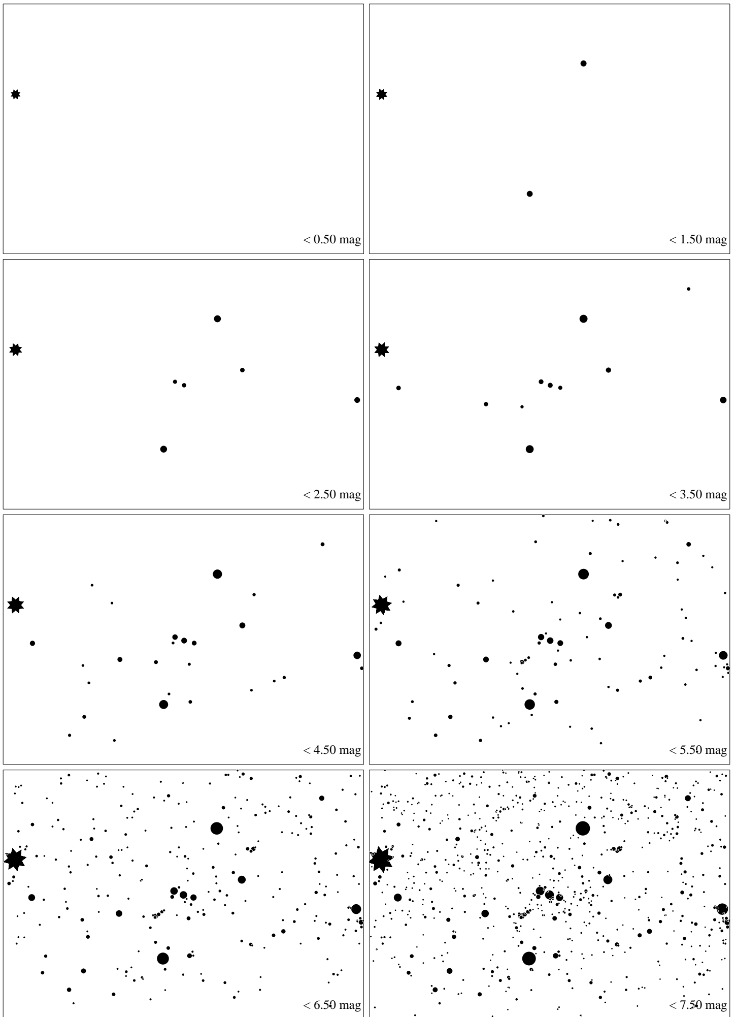
Maps for GLOBE at Night at latitude 30^\circ , March 30, 21 h local time (Mar 7, 22.5 h; Mar 23, 21.5 h, Apr 6, 20.5 h). Orion's belt is 72^\circ to the right from the south, at 26^\circ height. The brightest fixed star, Sirius, is at left. Jan Hollan, Ecological Institute Veronica and http://www.astro.cz/darksky
