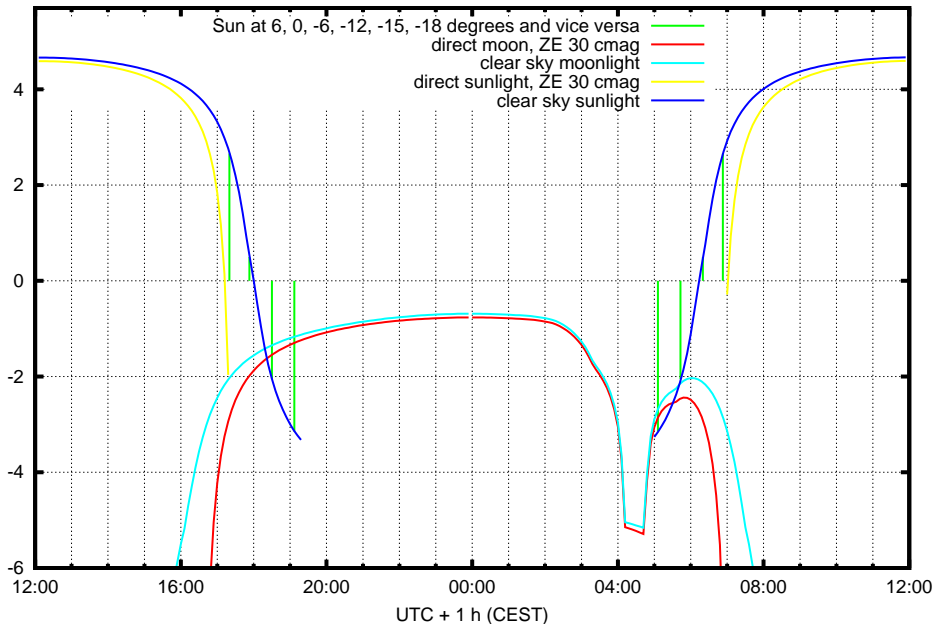
log 10 ( illuminance / 1 lx ) Kravi hora, Brno, ending at Thursday 2008-02-21 noon
