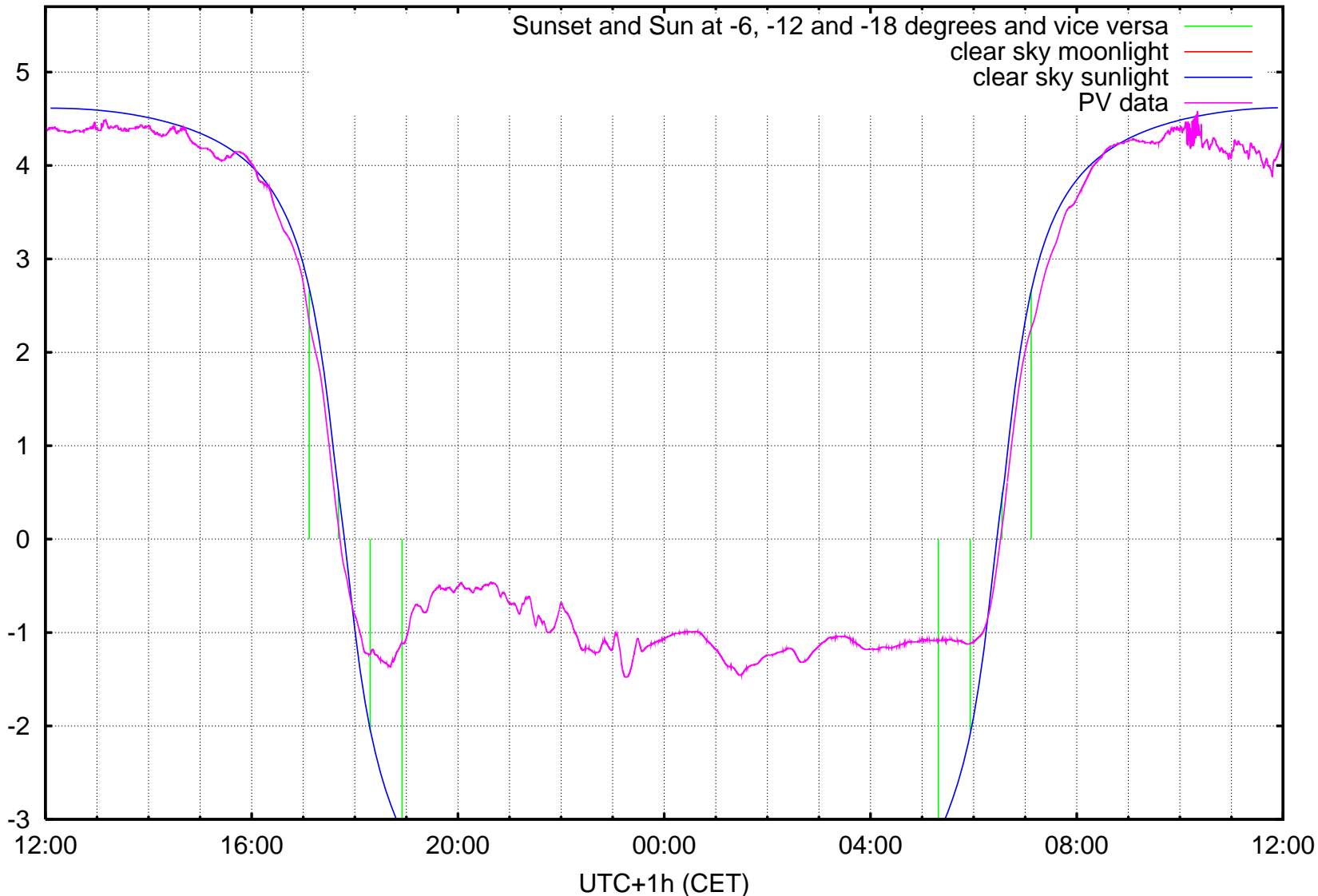
log10 ( illuminance / 1 lx ) Kravi hora, Brno, ending at Tuesday 2007-02-13 noon
