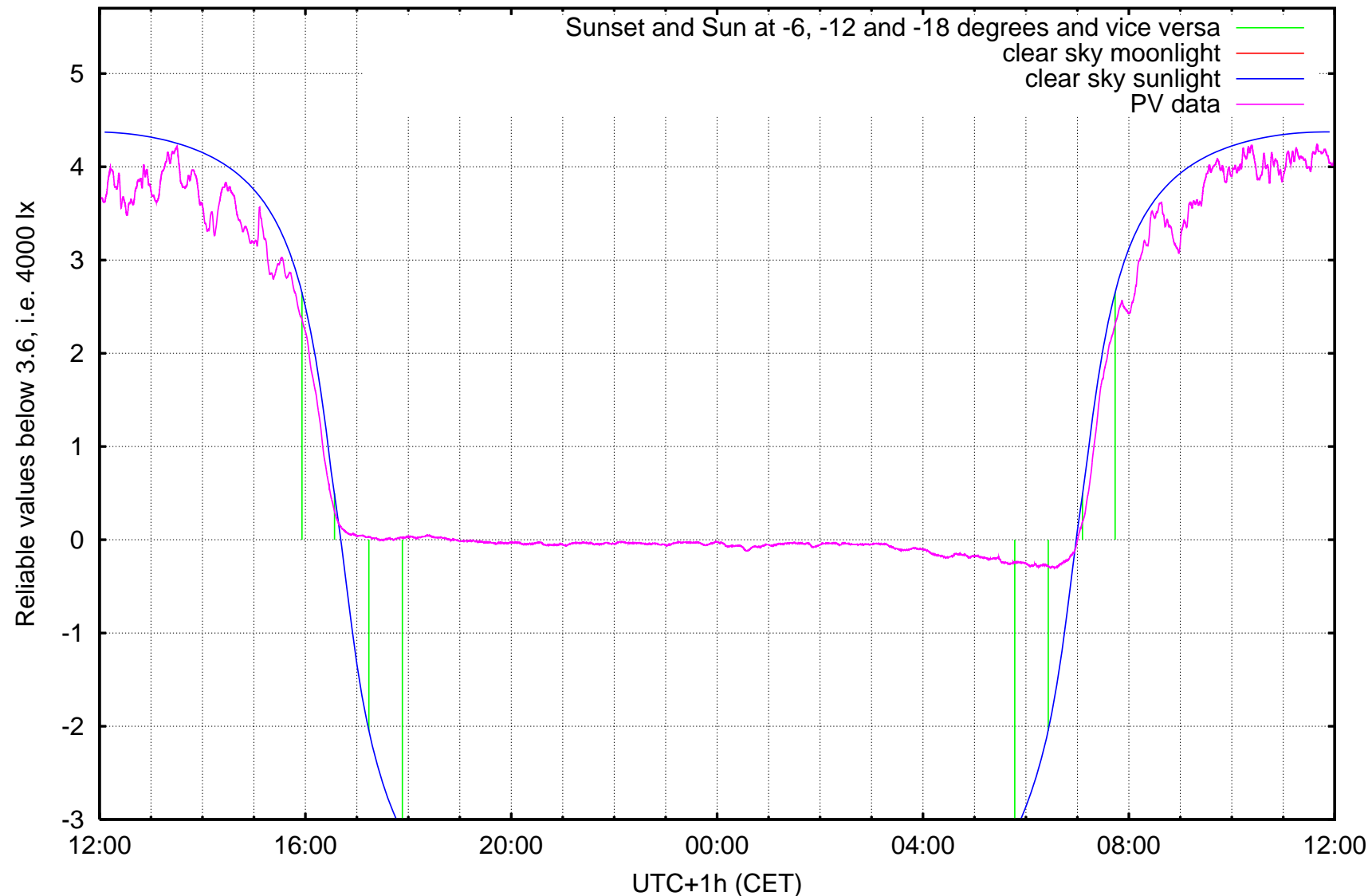
log10 ( illuminance / 1 lx ) Kravi hora, Brno, ending at Monday 2006-12-18 noon
