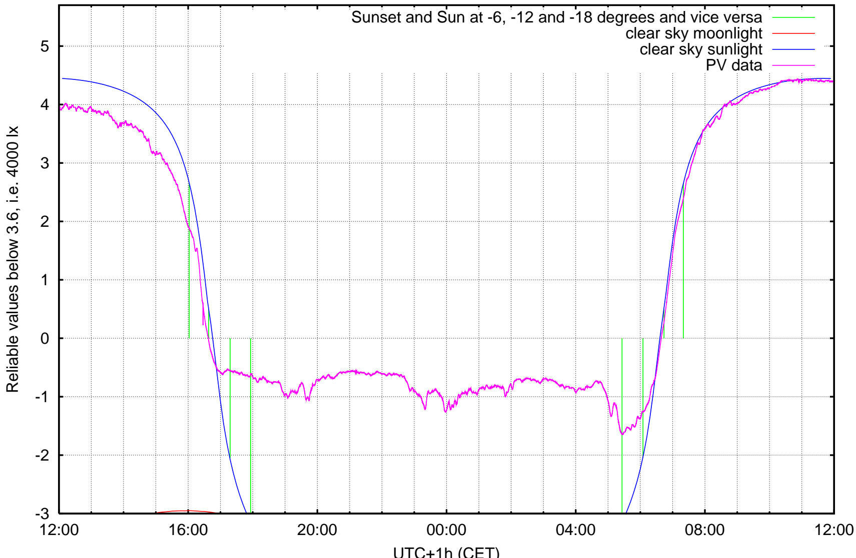
log10 ( illuminance / 1 lx ) Kravi hora, Brno, ending at Sunday 2006-11-26 noon
