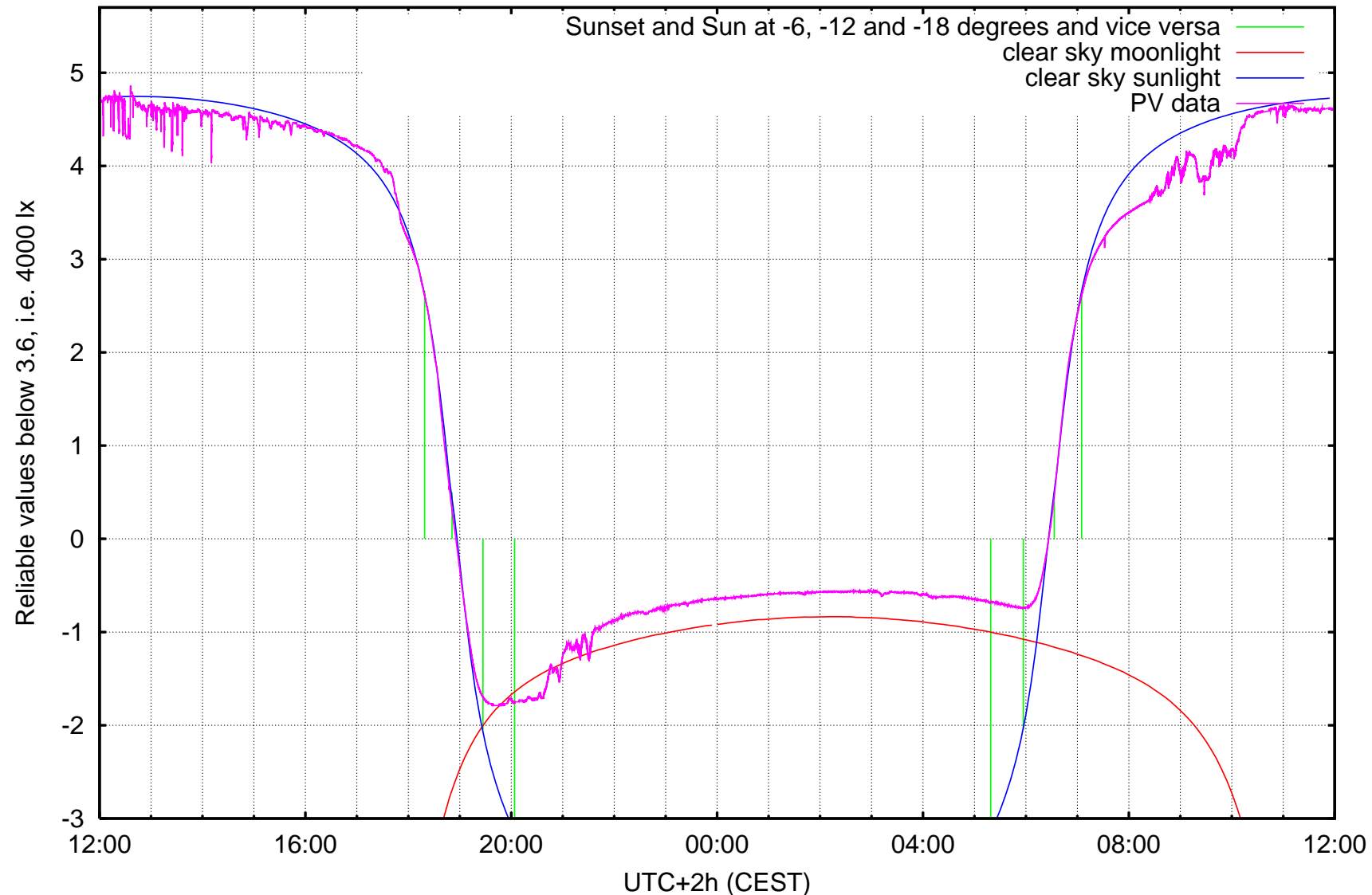
log10 ( illuminance / 1 lx ) Kravi hora, Brno, ending at Monday 2006-10-09 noon
