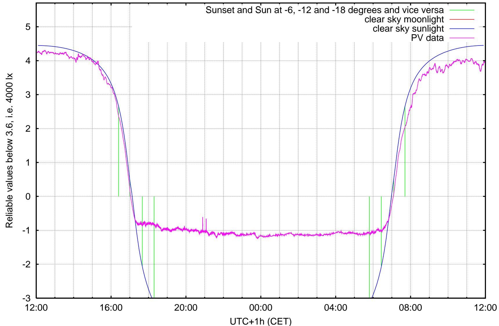
log10 ( illuminance / 1 lx ) Kravi hora, Brno, ending at Wednesday 2007-01-17 noon
