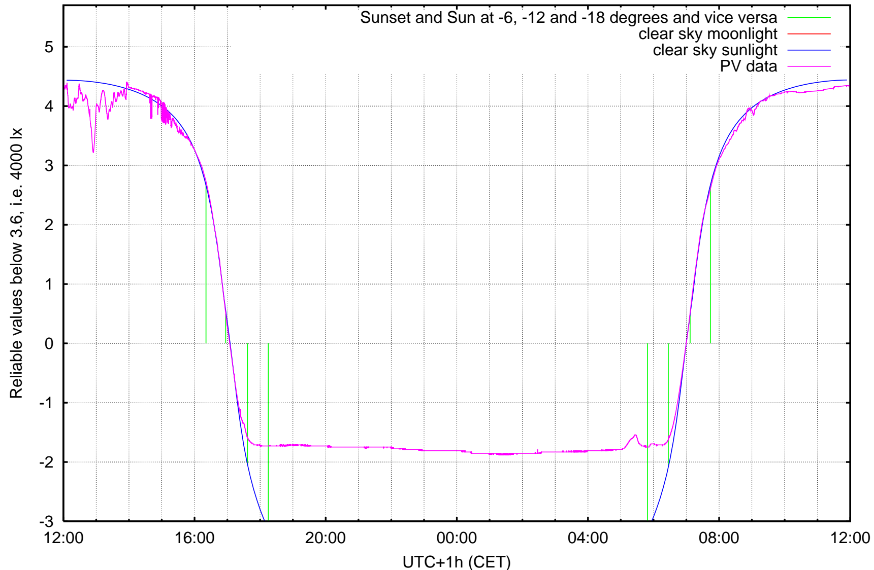
log10 ( illuminance / 1 lx ) Kravi hora, Brno, ending at Monday 2007-01-15 noon
