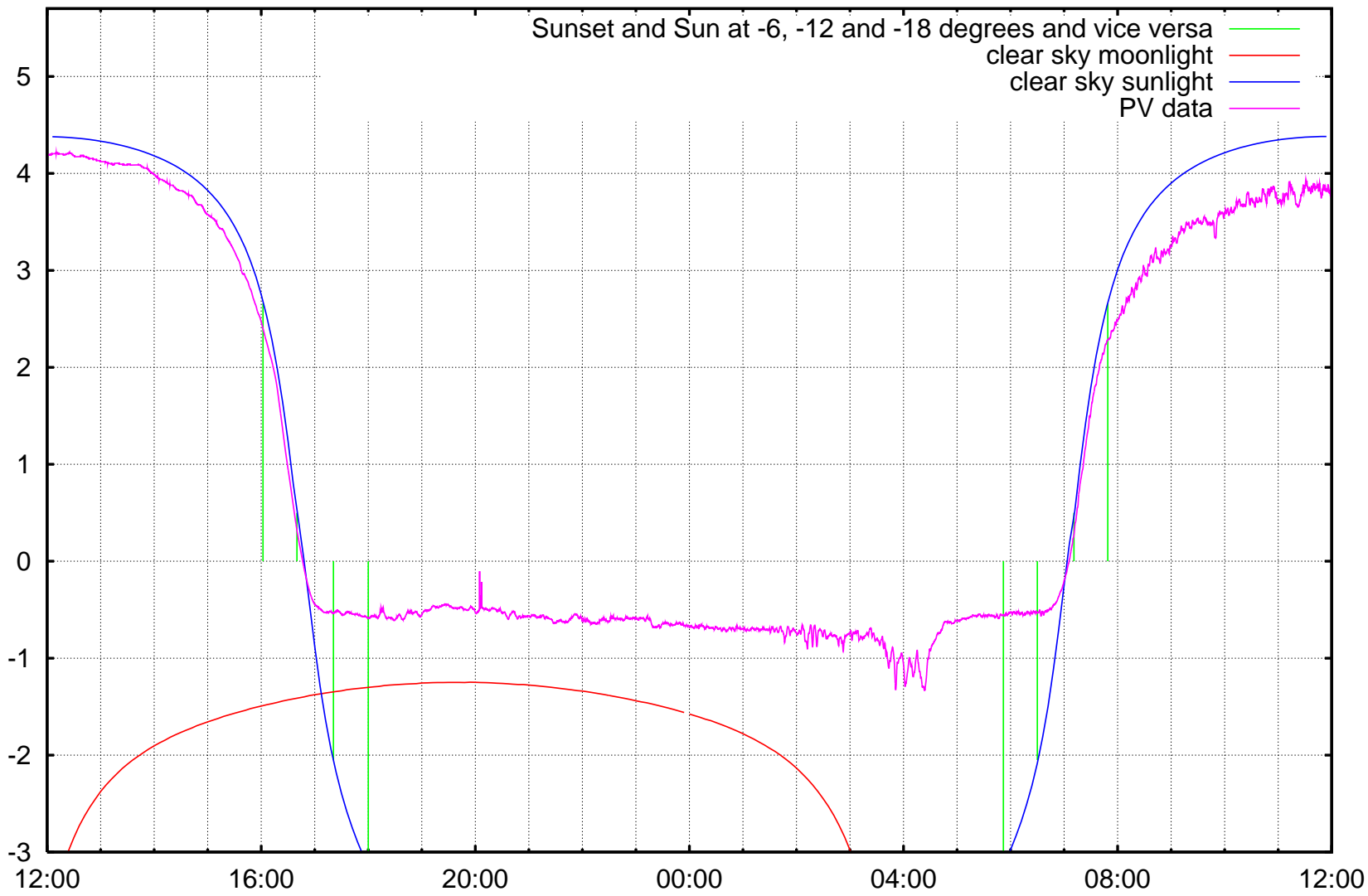
log10 ( illuminance / 1 lx ) Kravi hora, Brno, ending at Saturday 2006-12-30 noon
