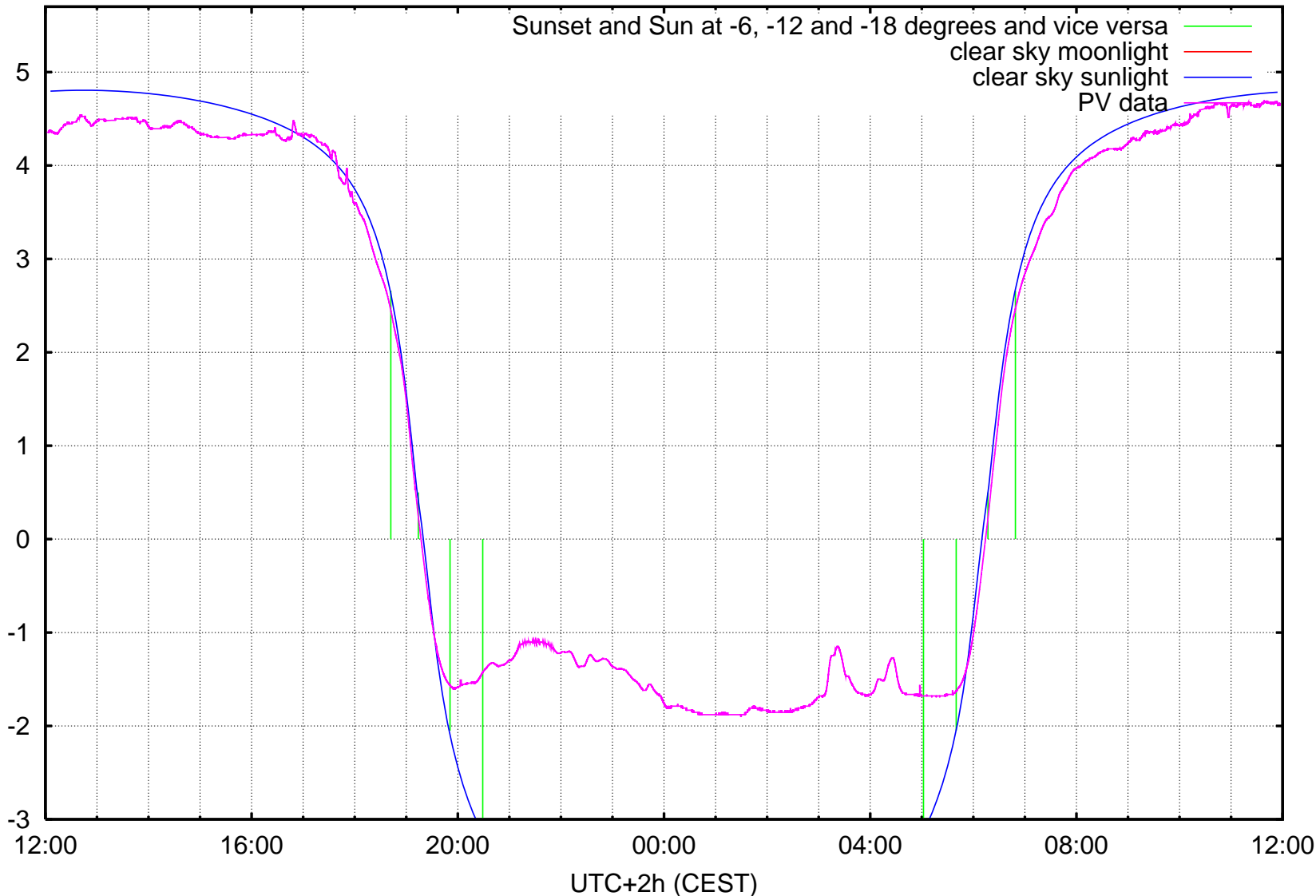
log10 ( illuminance / 1 lx ) Kravi hora, Brno, ending at Thursday 2006-09-28 noon
