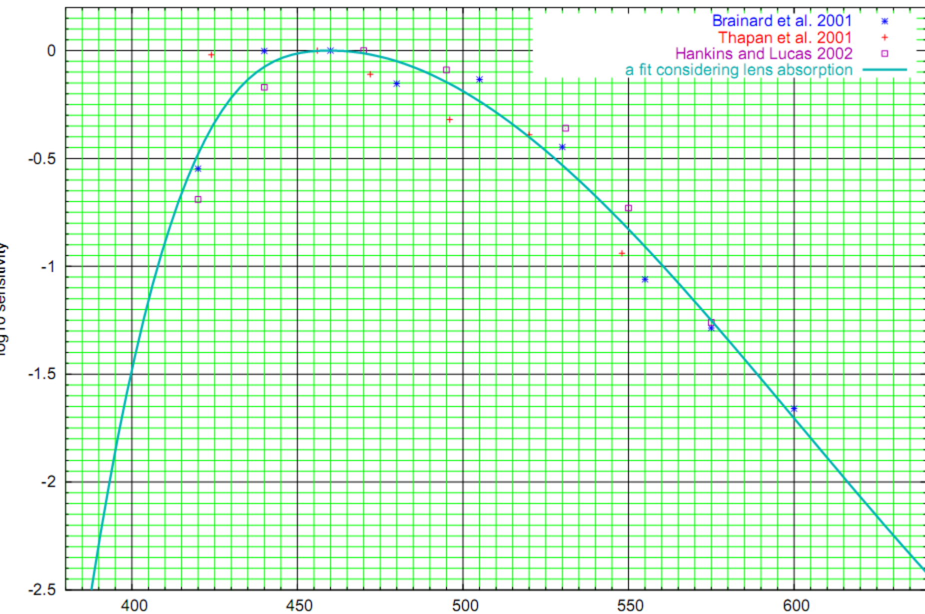
Action spectrum of melanonin suppression by light"
