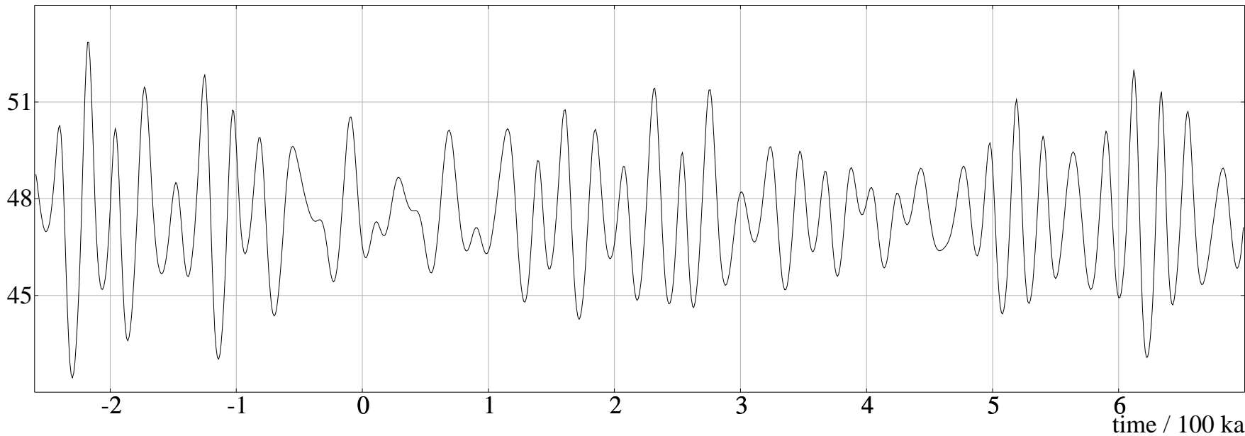
Mean insolation of 65N latitude during one month after the summer solstice
