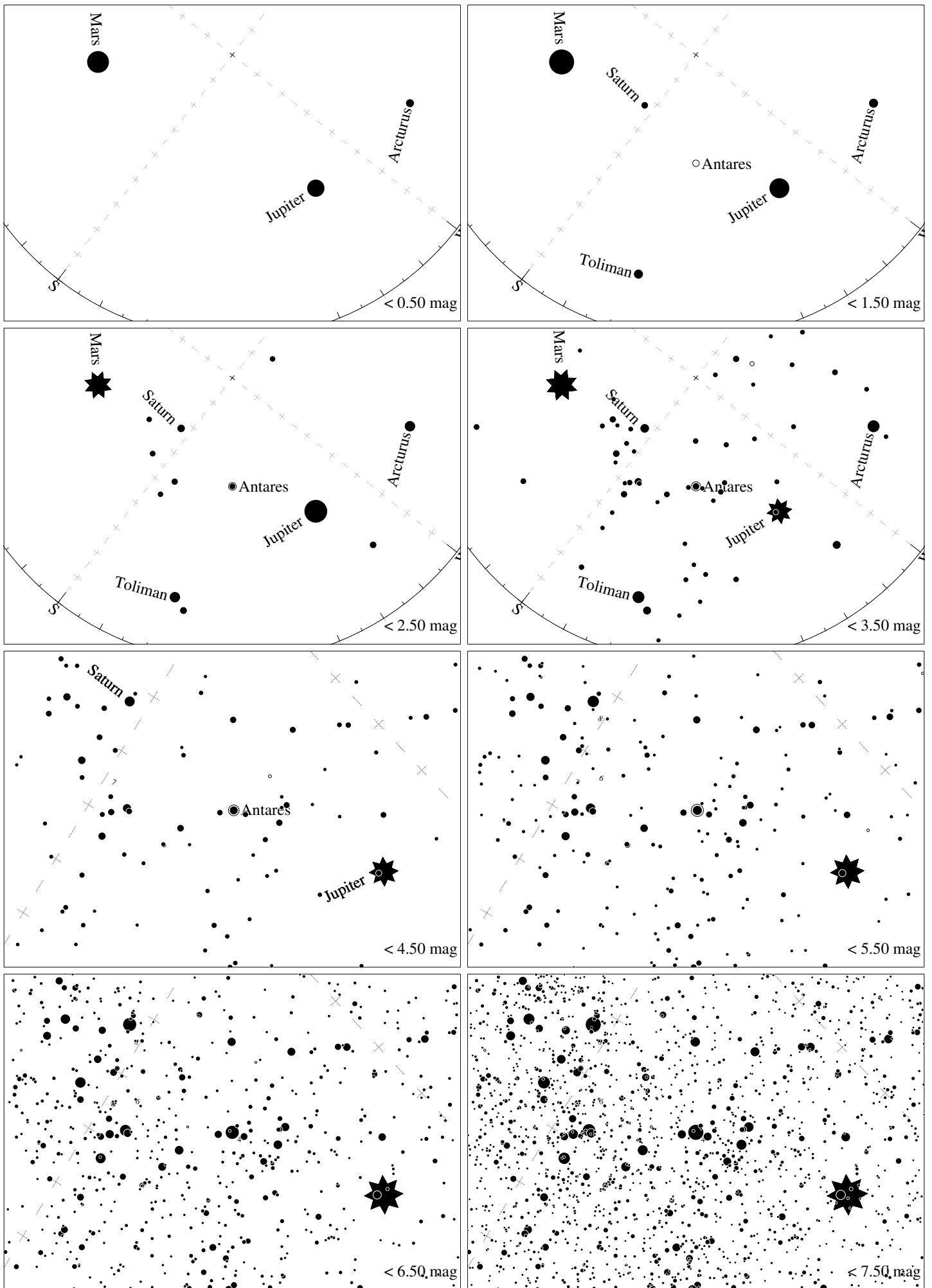
Maps for Globe at Night latitude 0°, 2018-08-06, 21 h local time (Sun at -41^\circ ), transparent air. Lines from N(E,S,W) to zenith shown (crosses each 10^\circ ). Centered on Antares ( \alpha Scorpii), which is 38^\circ to the right from S, at 56^\circ height. Detailed maps 50^\circ vertically, the first four maps 100^\circ . Jan Hollan, CzechGlobe
