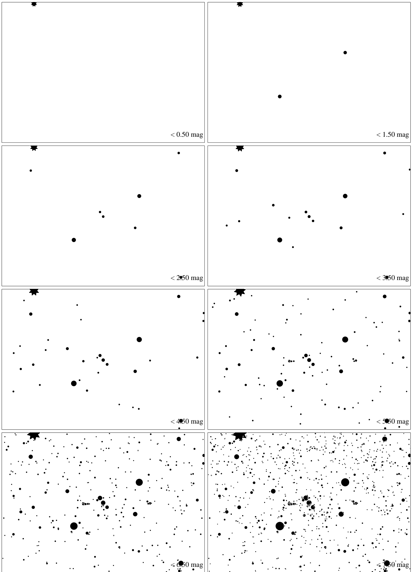
Maps for GLOBE at Night at latitude 0^\circ , March 30, 21 h local time (Mar 7, 22.5 h; Mar 23, 21.5 h, Apr 6, 20.5 h). Orion's belt is 89^\circ to the right from the south, at 31^\circ height. The brightest fixed star, Sirius, is at upper left. Jan Hollan, Ecological Institute Veronica and http://www.astro.cz/darksky
