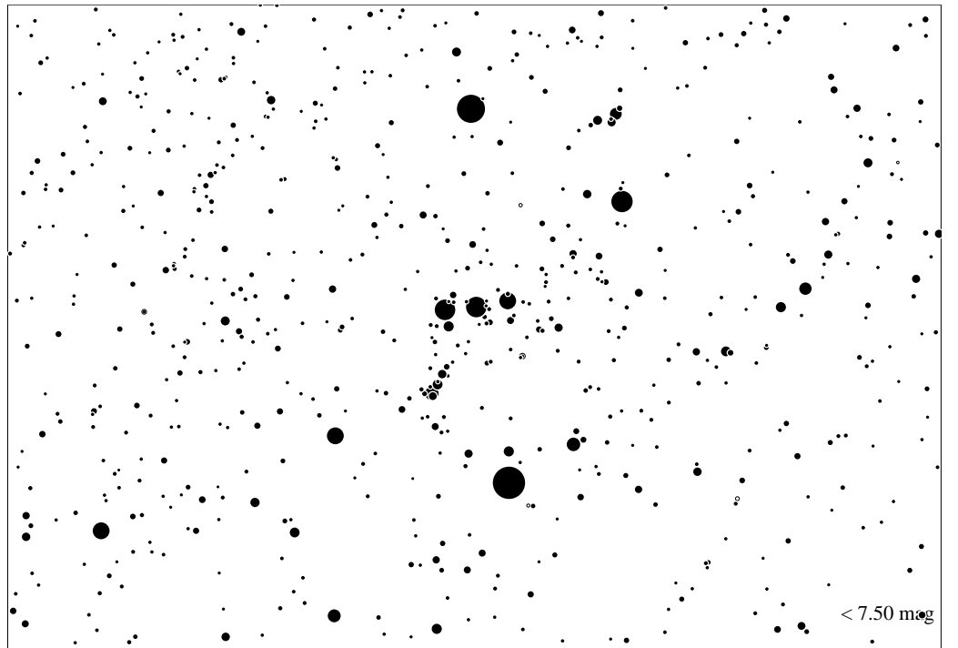
Maps for Globe at Night, lat. 49°, Mar 22, 2 h after sunset (20 h local mean time) = start of astronomical night. Orion's belt at 30°, Betelgeuze at 40°. Very clear air (extinction 0.20 mag in zenith). J. Hollan, N. Copernicus Observatory and Planetarium in Brno
