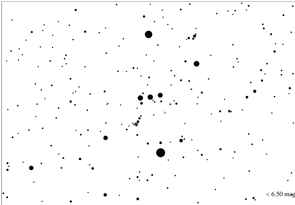
Maps for Globe at Night, lat. 49°, Mar 22, 2 h after sunset (20 h local mean time) = start of astronomical night. Orion's belt at 30°, Betelgeuze at 40°. Very clear air (extinction 0.20 mag in zenith). J. Hollan, N. Copernicus Observatory and Planetarium in Brno
