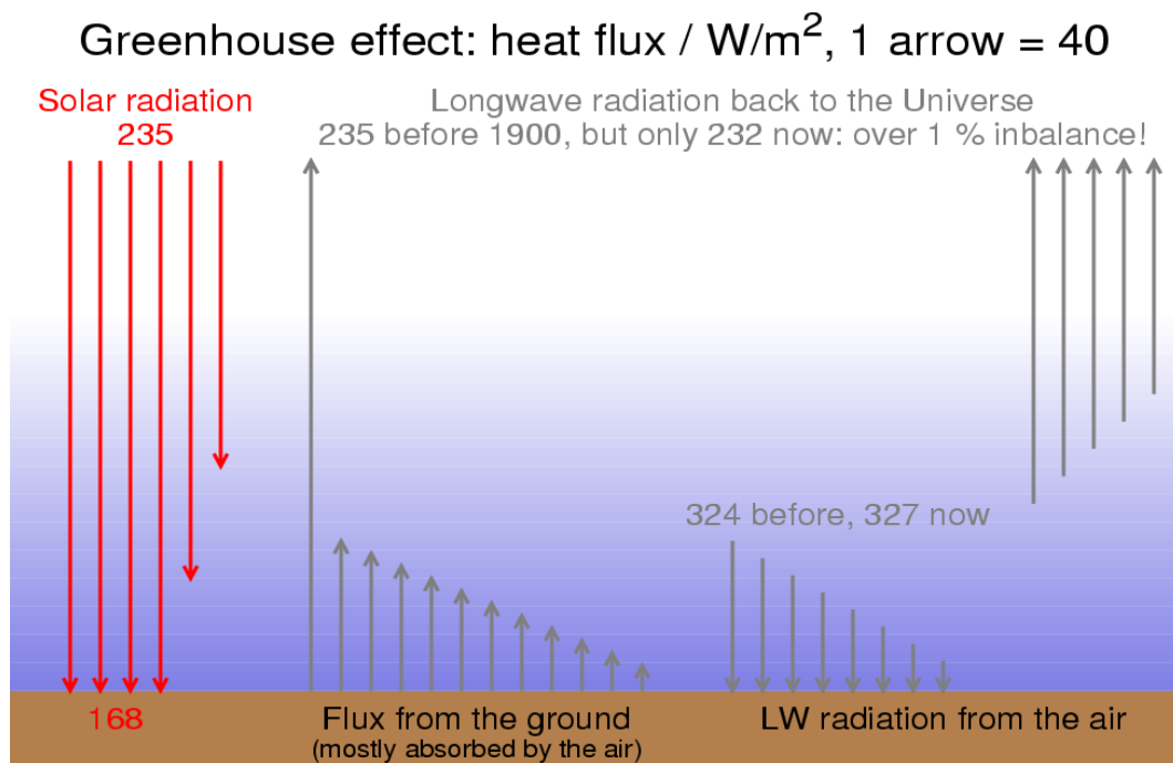
Figure 5: The huge invisible radiation fluxes; the radiative disbalance of 3 \text{ W/m}^2 ( 2 \text{ W/m}^2 more probably) might hold for a non-real case when no cooling aerosols would be produced by mankind
